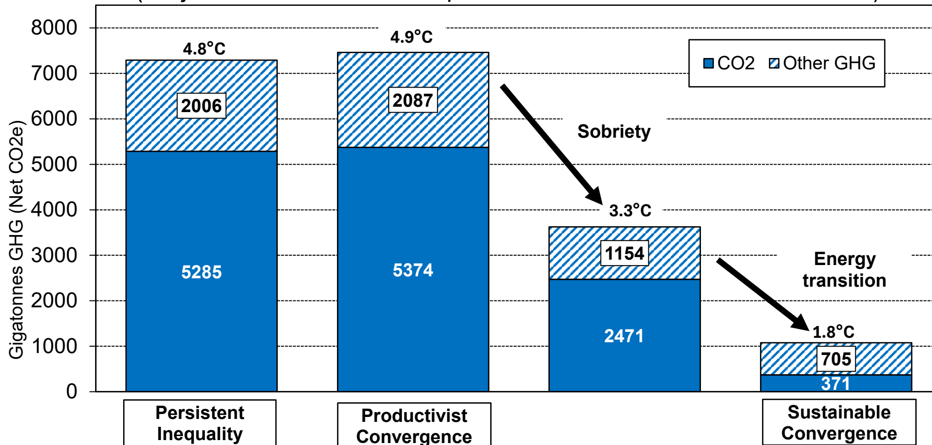
Fig. 44. Sobriety & Energy Transition Are Complementary (Projected Emissions & Temperature of Core Scenarios 2026-2100)
