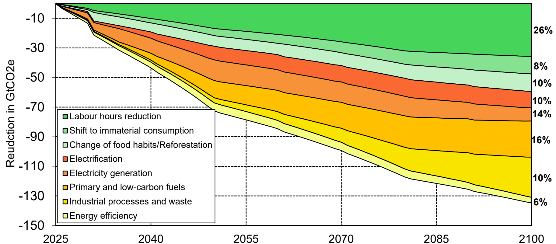
Fig. 46. Sobriety & Energy Transition Are Complementary (Decomposition of Emissions Reduction Drivers 2026-2100)
