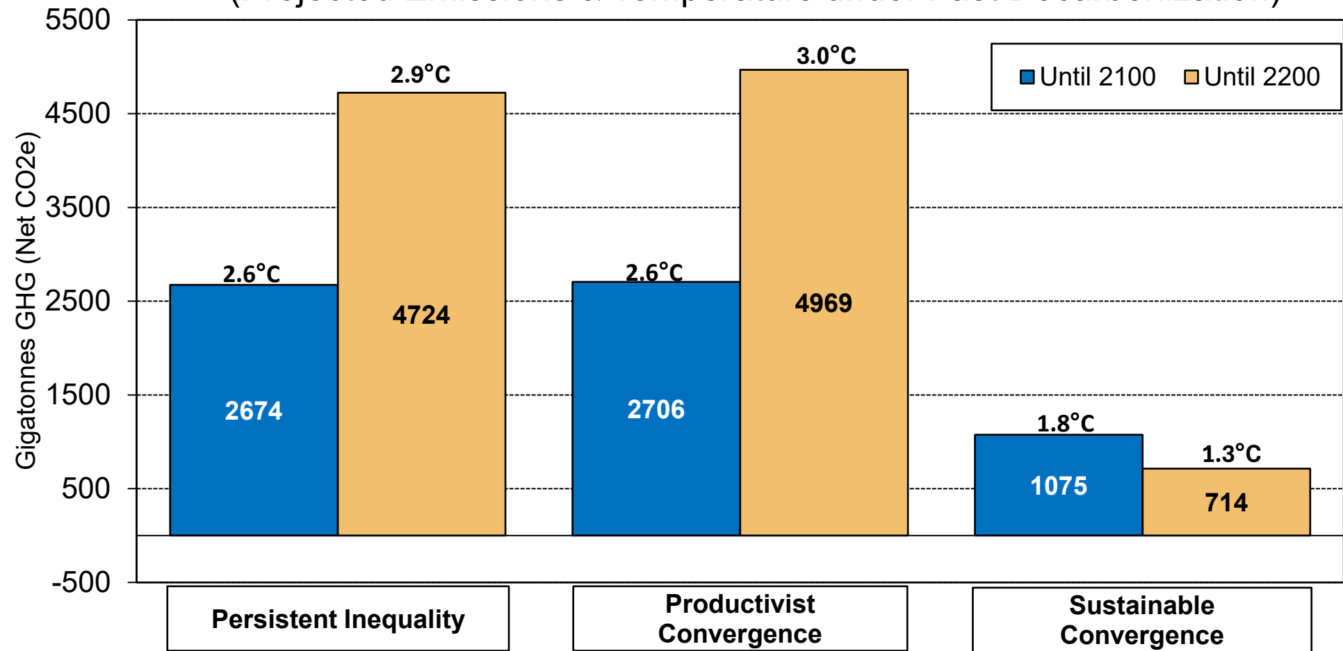
Fig. 48. Without Sobriety, Emissions Will Continue After 2100 (Projected Emissions & Temperature under Fast Decarbonization)
